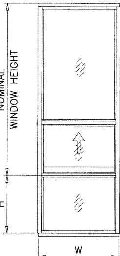
UNEQUAL LITES (ORIEL) SINGLE HUNG OVER FIXED WINDOWS
