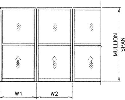
EQUAL LITES UNEQUAL LITES (ORIEL) SINGLE HUNG WINDOWS
