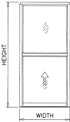
EQUAL LITES UNEQUAL LITES (ORIEL) SINGLE HUNG WINDOWS
