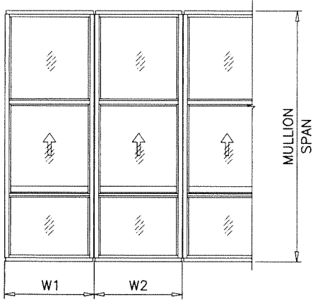
EQUAL LITES UNEQUAL LITES (ORIEL) SINGLE HUNG OVER FIXED WINDOWS
